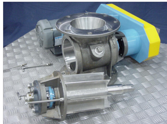
Rotor Released
