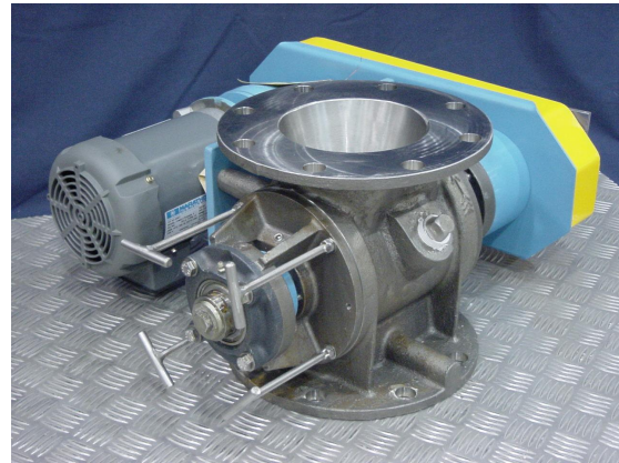
Drive Side View
